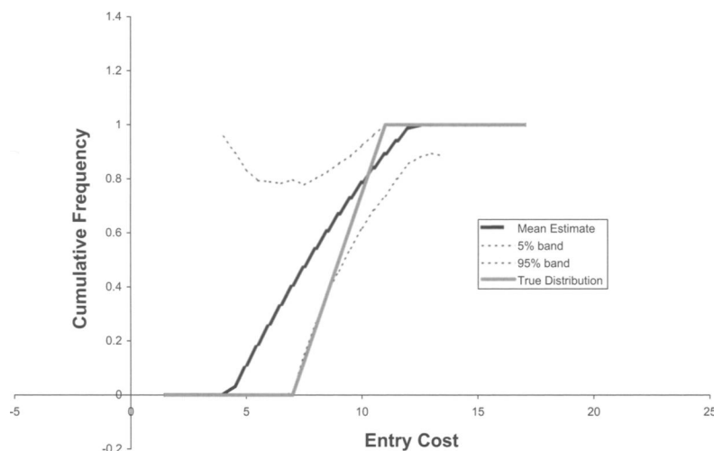
FIGURE 3.—Entry cost distribution for n = 100 .
