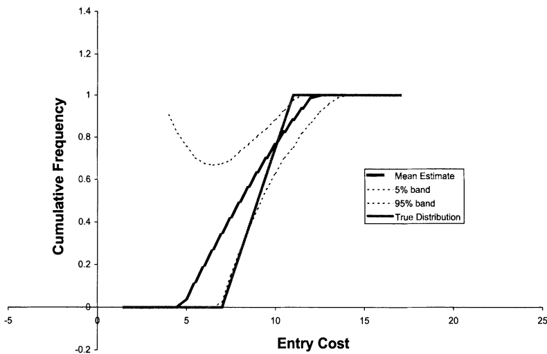
FIGURE 2.—Entry cost distribution for n = 200 .
